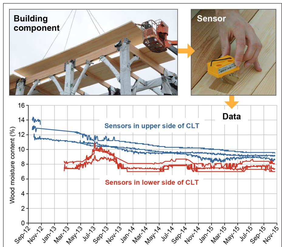
Figure 1. Easy-to-deploy wireless moisture sensor and example monitoring data.
