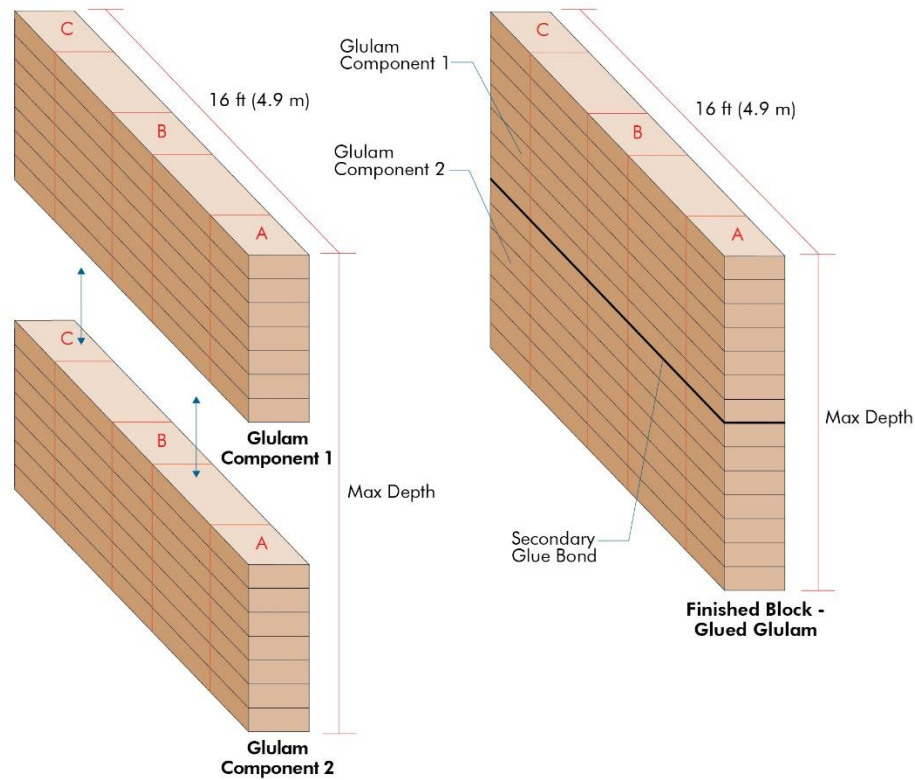
Figure 1. Block-Gluing on the Face of Glulam Components (drawing not to scale)
