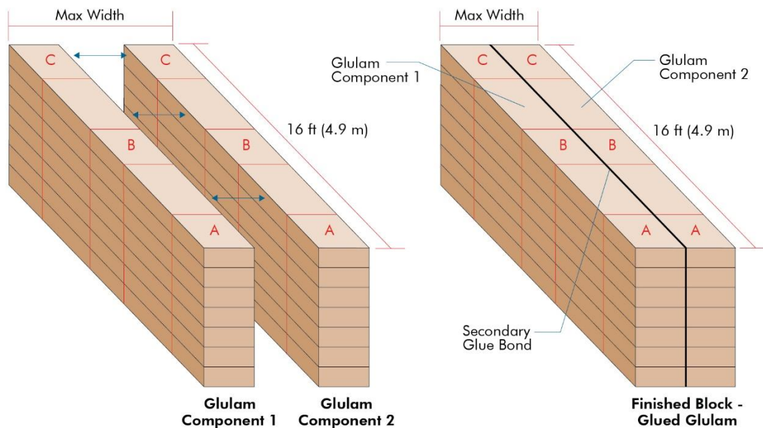
Figure 2. Block-Gluing on the Edge of Glulam Components (drawing not to scale)
